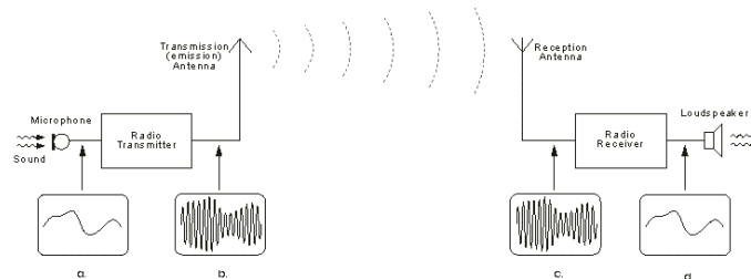
Fig. 2.1. Radio Transmission Block-Diagram
